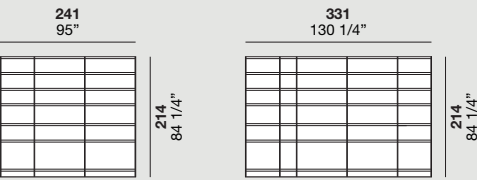
dispensa scaffale pantry shelf unit
