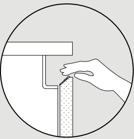
LOGICA L40 apertura con gola curva / profilo L40 opening with curved groove and L40 profile
