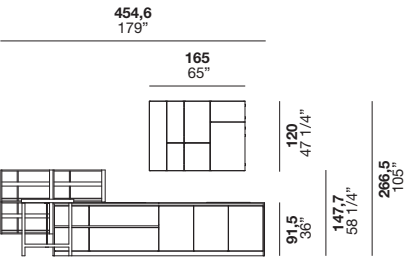
pensili / basi wall units / base units
