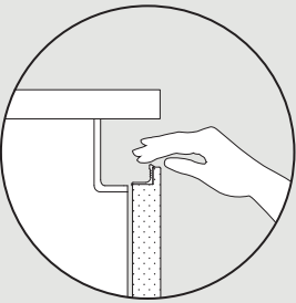
LOGICA L90 apertura con gola curva / profilo L90 opening with curved groove and L90 profile
