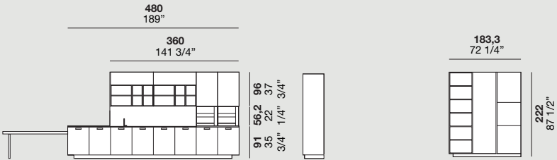
tavolo Axia Axia table pensili a giorno / basi / pass open wall units / base units / pass colonne tall units
